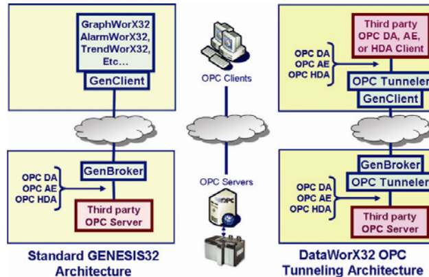
DataWorX32 OPC Tunneler Architecture
