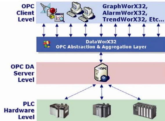
Architecture of OPC Data Aggregation
